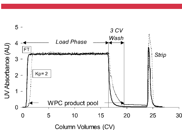
Figure 4. Chromatograms from column runs under flowthrough ( K_p < 0.1 ) and weak partitioning conditions ( K_p = 2 ) display the effects of increasing mAb K_p on the product breakthrough and washout regions of the chromatogram. The column strip peak is also larger, due to the increased removal of host cell proteins and a slight increase in product loss.
